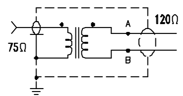
SCHMATIC DIAGRAM
