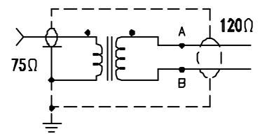
SCHMATIC DIAGRAM
