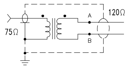
SCHMATIC DIAGRAM
